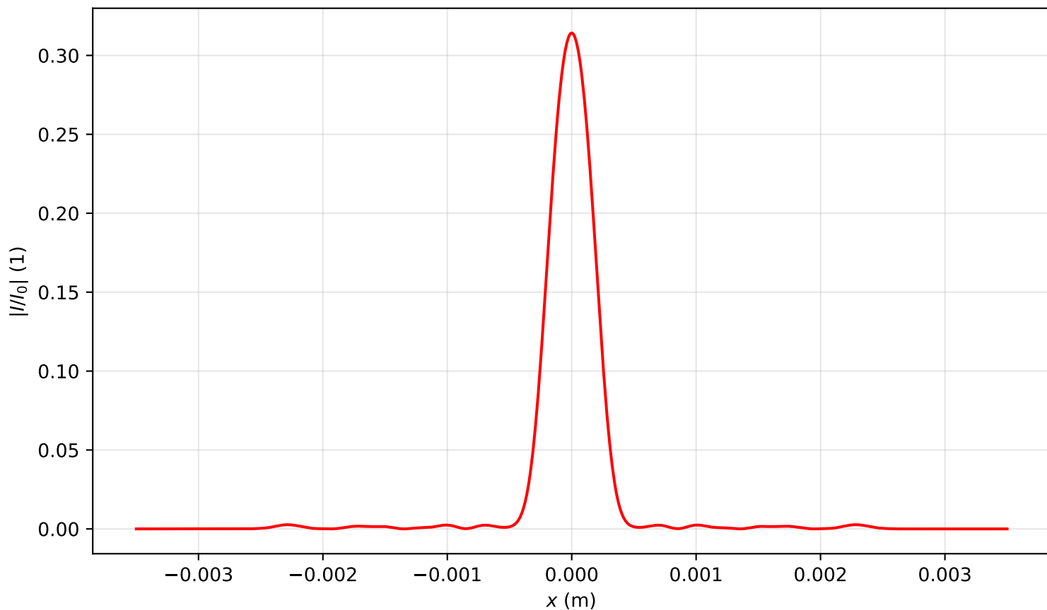
Intensity profile I(x, y = 0, z = 3.503)/I_0 , P_{in}=7.0P_{cr} , artificial time
